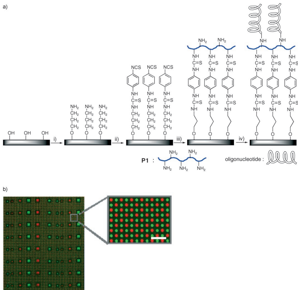
Figure 3. a) Schematic representation of the light-directed parallel on-chip DNA synthesis on P1 -immobilized glass: i) APTMS, ii) 1,4-phenylenediisothiocyanate, iii) polymer ( P1 ), and iv) cyclic procedures of oligo synthesis. b) A fluorescence image of a patterned signal-amplifying DNA microarray with two different DNA sequences after hybridization with a mixture of c-DNA-HEX (green) and c-DNA-Cy5 (red; scale bar: 200 \mu\text{m} ).
